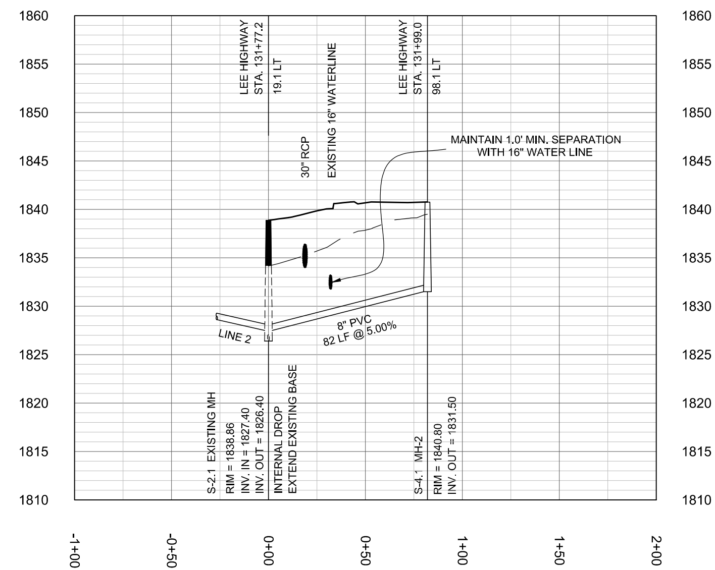
SEWER LINE 4
