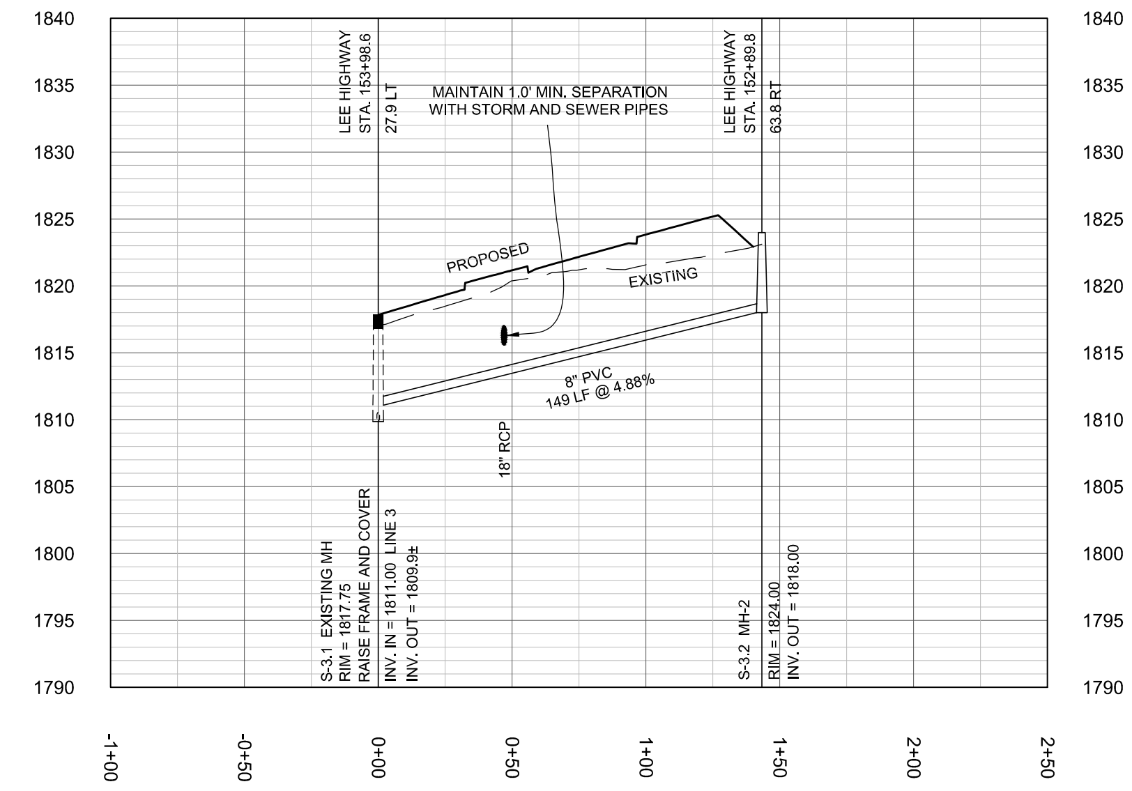
SEWER LINE 3
