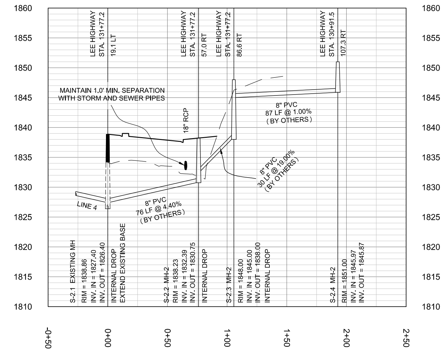
SEWER LINE 2 ( BY OTHERS )
