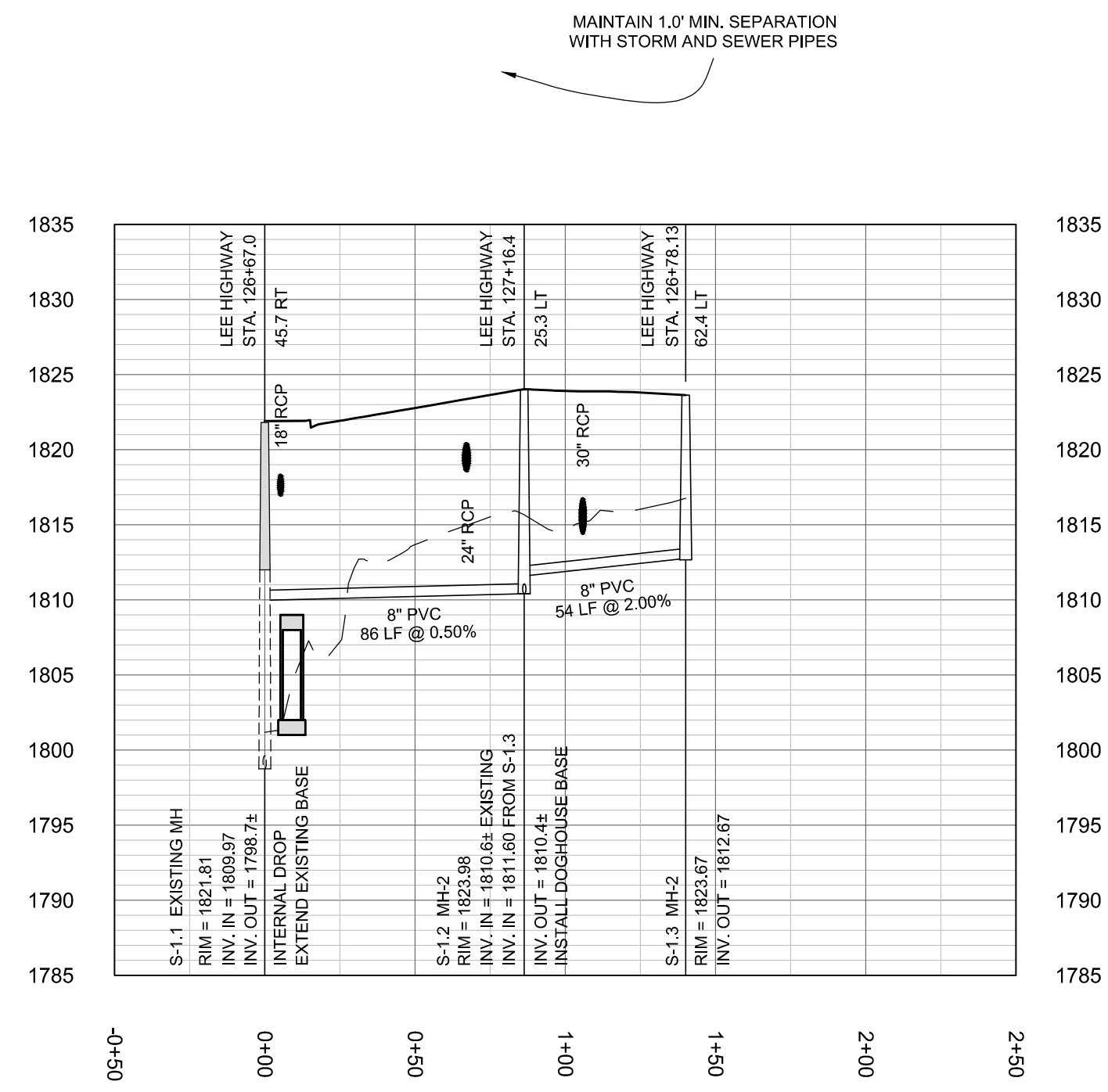
SEWER LINE 1
